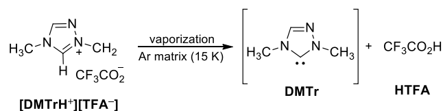
Scheme 6. Thermal decomposition of [DMTrH + ] [TFA - ] during vaporization (~333 K) and subsequent isolation of vapors in an Ar matrix at 15 K, which leads to the formation of carbene DMTr (not identified) and HTFA.
