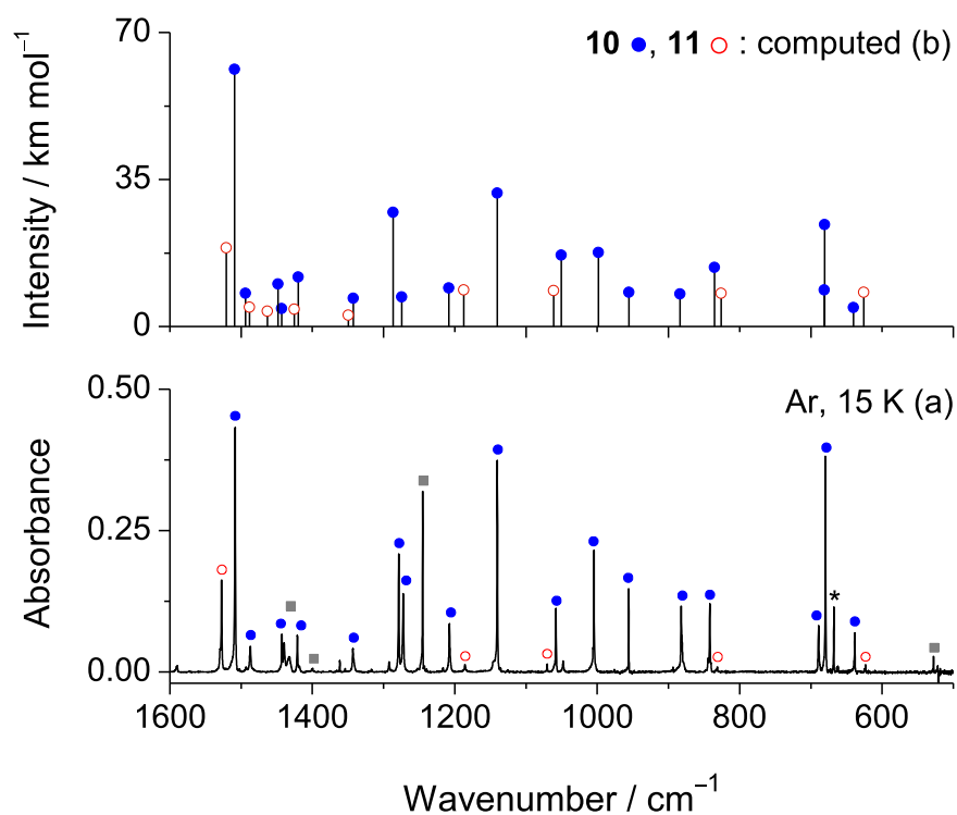
Fig. 3. (a) Experimental IR spectrum of the vapors of [\text{DMTrH}^+][\text{I}^-] trapped in an Ar matrix at 15 K. Bands marked with closed blue circles and open red circles are assigned to 10 and 11 , respectively, based on comparison with their corresponding computed spectra. Bands assigned to methyl iodide 12 are marked with grey squares, with their identification based on the IR spectrum of the compound isolated in an Ar matrix [46]. The band at 668 \text{cm}^{-1} , marked with an asterisk (*), is due to atmospheric \text{CO}_2 . (b) B3LYP/6-311+G(2d,p) computed IR spectrum of 1-methyl-1H-1,2,4-triazole 10 (closed blue circles) and 4-methyl-4H-1,2,4-triazole 11 (open red circles). The IR intensities of 11 were scaled by 0.3 to provide a 10 : 11 ratio of 1:0.3 that better reproduces the experimental data. Only bands with computed IR intensities > 2 \text{ km mol}^{-1} are shown.
