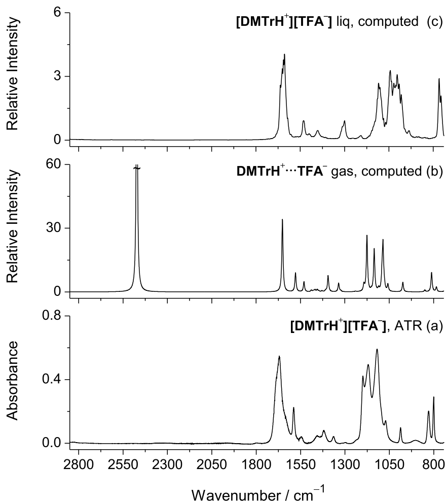
Fig. 4. (a) Experimental IR spectrum (ATR) of [\text{DMTrH}^+][\text{TFA}^-] as pure liquid at room temperature. (b) B3LYP/6-311+G(2d,p)-GD3BJ computed IR spectrum of the most stable [\text{DMTrH}^+\cdots\text{TFA}^-] ion pair (I). (c) Theoretical IR spectrum of the [\text{DMTrH}^+][\text{TFA}^-] ionic liquid obtained from AIMD simulations.
