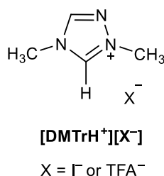
Scheme 4. Representation of the 1,2,4-triazolium salts studied in the present work: 1,4-dimethyl-4H-1,2,4-triazolium iodide [DMTrH + ][I - ] and 1,4-dimethyl-4H-1,2,4-triazolium trifluoroacetate [DMTrH + ][TFA - ].
