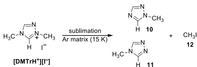
Scheme 5. Thermal decomposition of [DMTrH + ][I - ] during its sublimation (~363 K) and subsequent isolation of the vapors in an Ar matrix at 15 K, which leads to the formation of 1-methyl-1 H -1,2,4-triazole 10 , 4-methyl-4 H -1,2,4-triazole 11 , and CH 3 I 12 .
