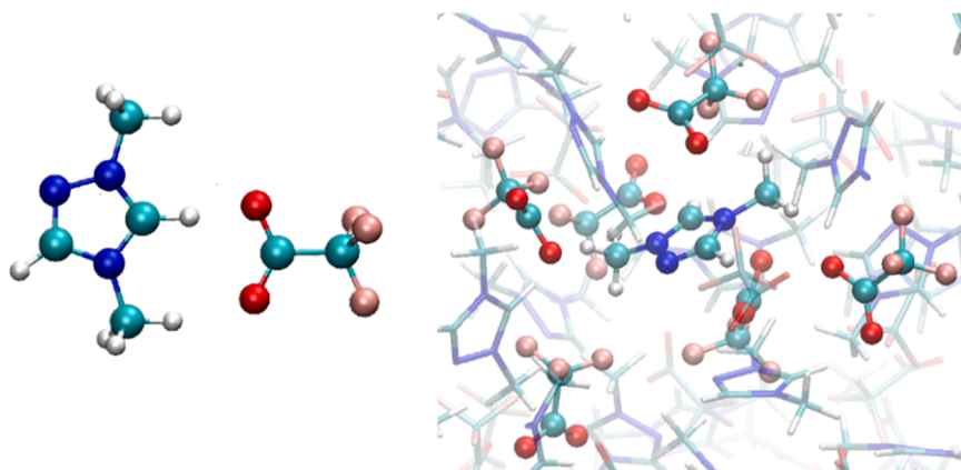
Fig. 5. Left: Computed structure of most stable [\text{DMTrH}^+\cdots\text{TFA}^-] ion pair (I) in gas-phase. Right: Snapshot of the Molecular Dynamics simulation trajectory computed for the bulk liquid [\text{DMTrH}^+][\text{TFA}^-] .
