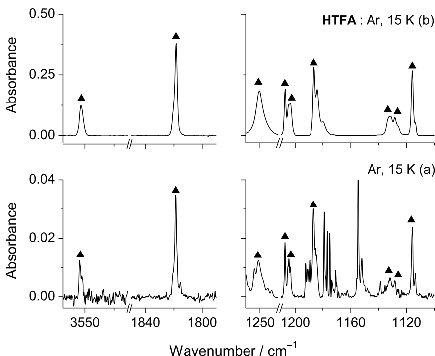
Fig. 6. (a) Selected regions of the experimental IR spectrum of the vapors of [DMTrH + ] [TFA - ] trapped in an Ar matrix at 15 K. Triangles indicate IR bands assigned to trifluoroacetic acid HTFA. (b) Selected regions of the experimental IR spectrum of an authentic sample of HTFA deposited in an Ar matrix at 15 K [51].
