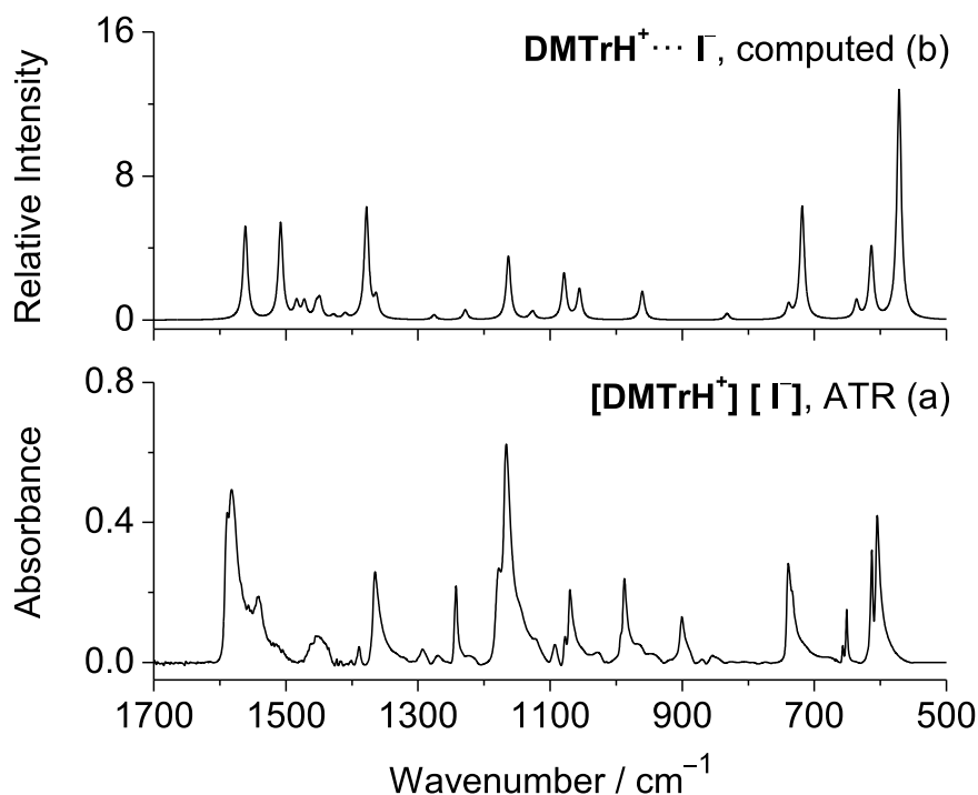
Fig. 2. (a) Experimental ATR IR spectrum of [\text{DMTrH}^+][\text{I}^-] at room temperature. (b) B3LYP/6-311+G(2d,p)[LANL2DZ]-GD3BJ computed IR spectrum of the [\text{DMTrH}^+ \cdots \text{I}^-] ion pair.
