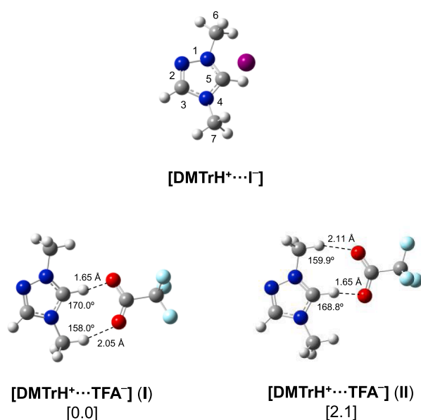
Fig. 1. B3LYP/6–311+G(2d,p)[LANL2DZ]-GD3BJ optimized geometry of the [\text{DMTrH}^+\cdots\text{I}^-] ion pair (atom numbering is given for the 1,2,4-triazolium cation) and B3LYP/6–311+G(2d,p)-GD3BJ optimized geometries of the two most stable minima (labelled as I and II) of the [\text{DMTrH}^+\cdots\text{TFA}^-] ion pair (values in square brackets are the relative Gibbs energies at 298.15 K in kJ mol ^{-1} ). The geometric parameters refer to the H \cdots O distances (Å) and C–H \cdots O angles (°) for the hydrogen bonds formed.
