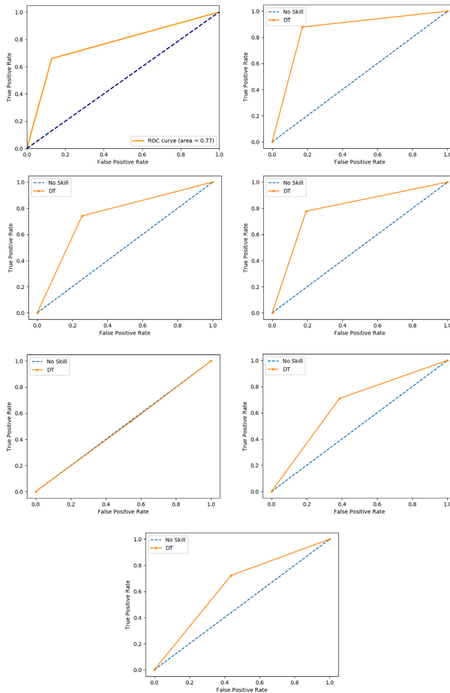
Fig. 3. Decision tree ROC curves.
