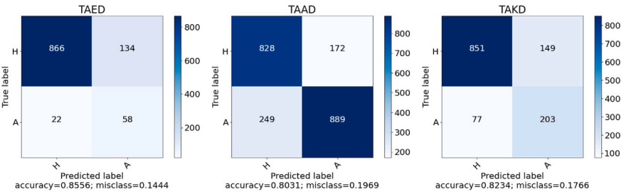
Fig. 8. Confusion matrices of (a) TAED, (b) TAAD, and (c) TAKD.
