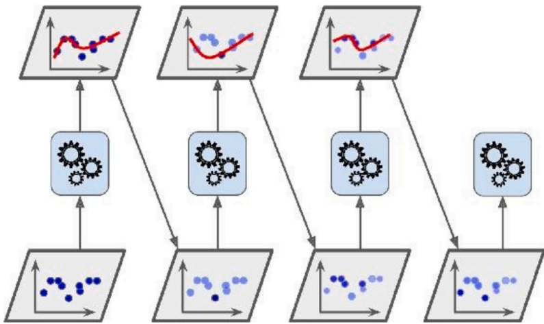
Fig. 6. Boosting structure.
