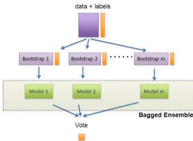
Fig. 5. Bagging structure.
