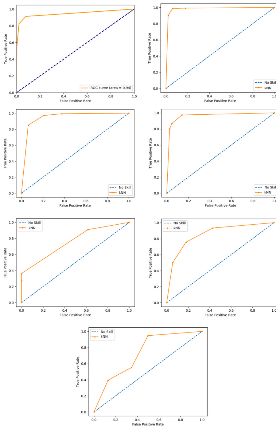
Fig. 4. kNN ROC curves.
