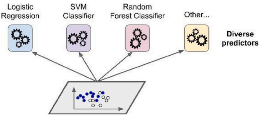
Fig. 7. Voting structure.
