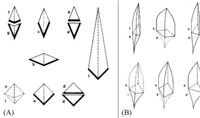
Figure 1. (A) Ceiling elements drawn according to Al-Kashi's descriptions; (B) 3D elements of muqarnas (Özdural, 1990, p. 38- 40).
