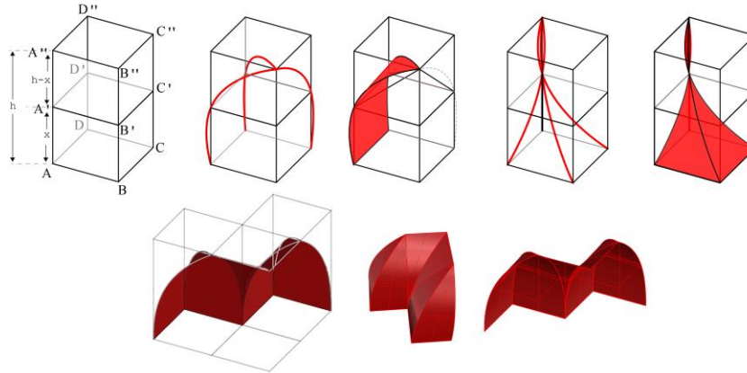
Figure 5. Modelling exercise of a muqarnas unit.
