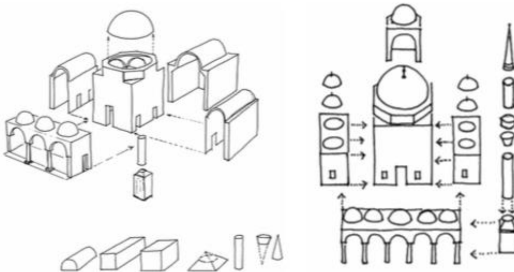
Image 1. Components of Classical Ottoman Mosque [5]
