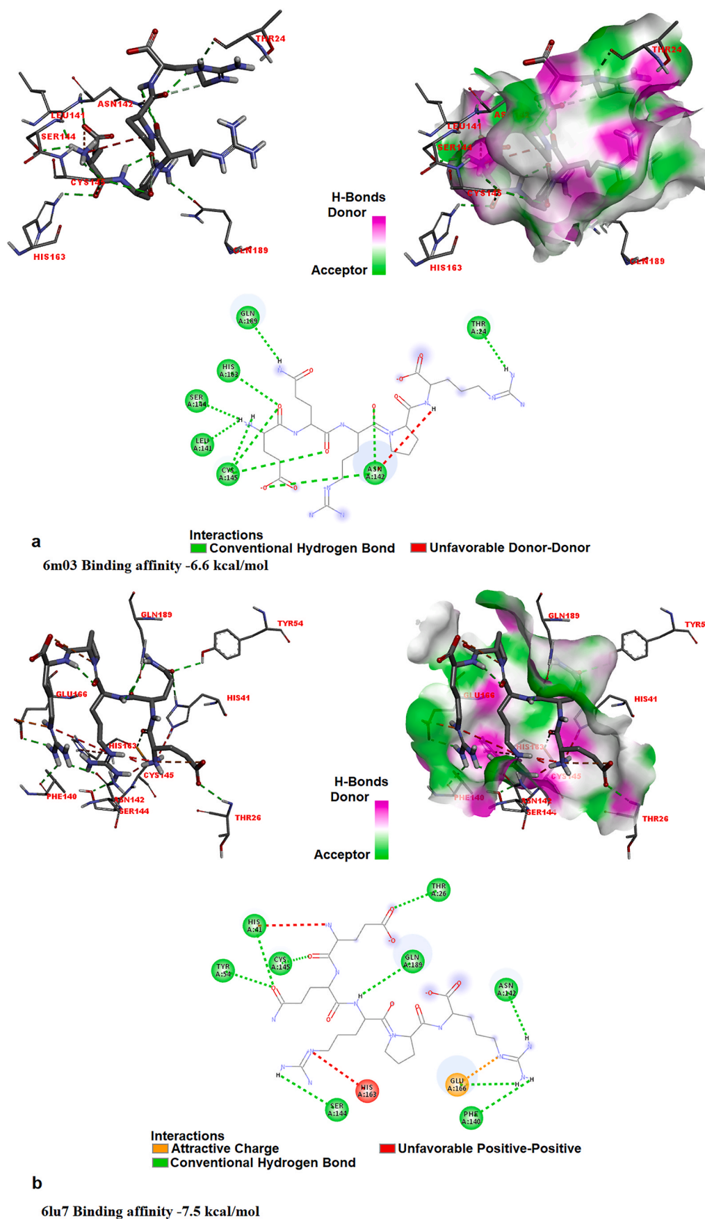
Fig. 6. The 3D docked views of the most stable conformer of EQRPR in Apo (a) and Holo (b) forms of MP pro . The ligand interaction diagrams of receptor-ligand complexes are shown.
