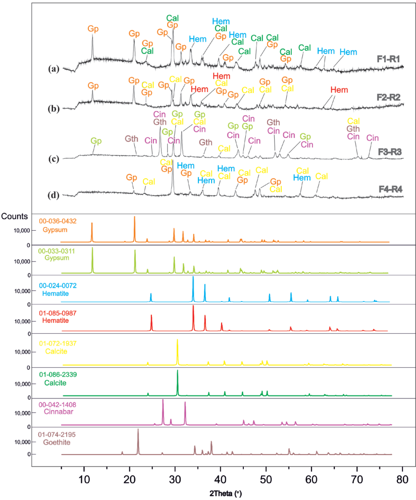
Figure 4. \mu -X-ray diffraction pattern of the bulk red samples' surface. Identified minerals: calcite (Cal), gypsum (Gp), hematite (Hem), goethite (Gth), quartz (Qz), cinnabar (Cin).
