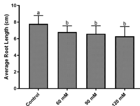
Figure 1. Effect of increasing NaCl concentrations on average root length of Osmancik-97 rice variety.
