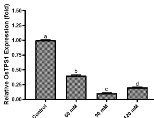
Figure 7. Effect of increasing NaCl concentrations on OsTPS1 gene expression of Osmancık-97 rice variety.
