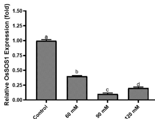
Figure 9. Effect of increasing NaCl concentrations on OsSOS1 gene expression of Osmancik-97 rice variety.
