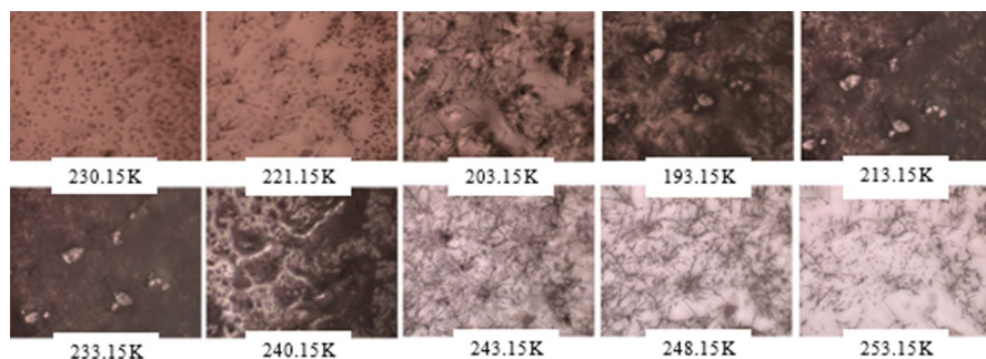
Fig. 7 Eutectic mixture photographs collected during the temperature-variation Raman spectroscopy experiment, with 10× magnification
