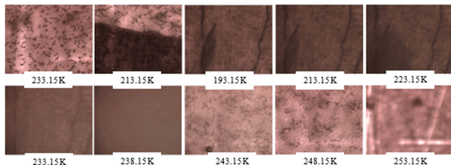
Fig. 8 80:20 diethyl adipate:dibutyl adipate mixture photographs collected during the temperature-variation Raman spectroscopy experiment, with 10× magnification
