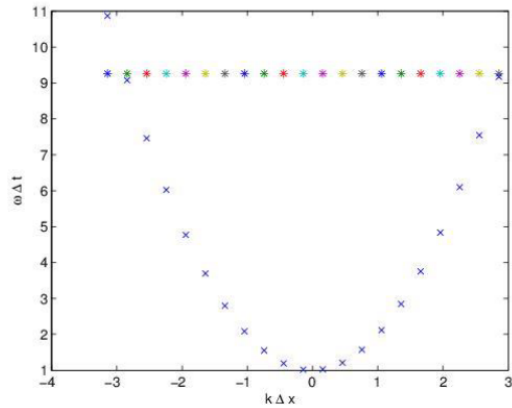
Figure 1. For \Delta t= \Delta x=0,1 , Exact (dot) and Numeric (solid) Dispersion Relation for Imaginary Part of Linearized Burgers-Huxley Equation
